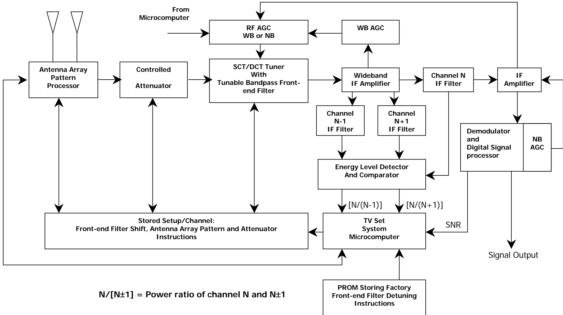
Figure 2: Schematic Diagram of the Processing and Control Circuits
